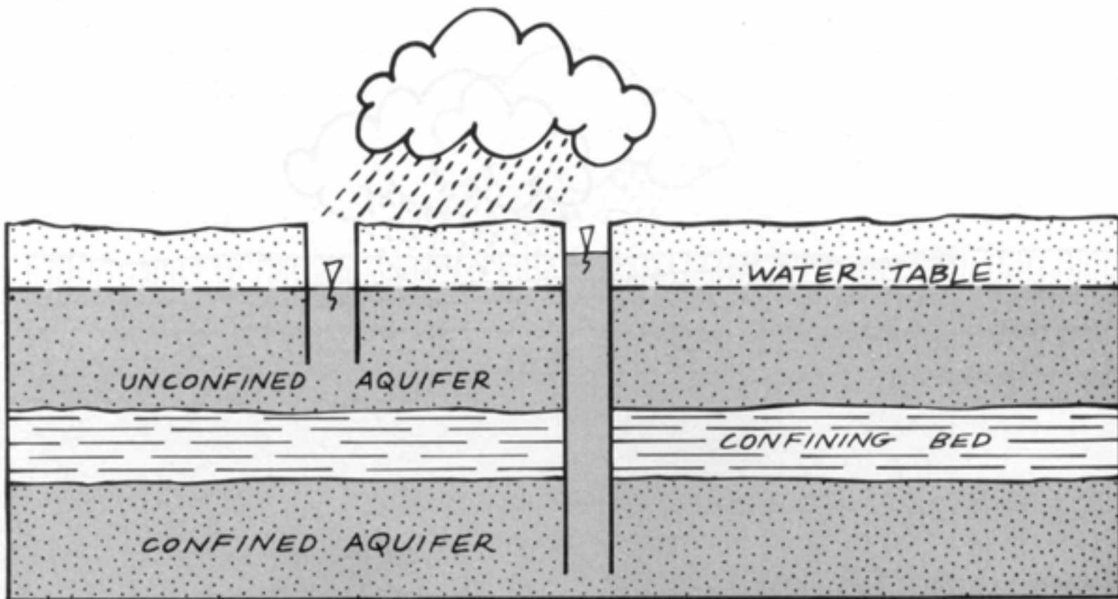
Figure 7.8 Typical occurrence of groundwater in confined and unconfined aquifers.
