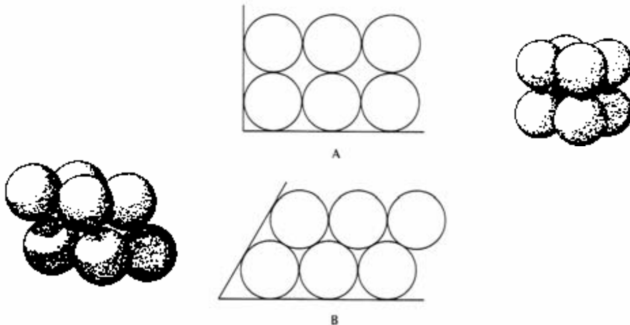
FIGURE 4.1 A. Cubic packing of spheres with a porosity of 47.65% B. Rhombohedral packing of spheres with a porosity of 25.95%.
